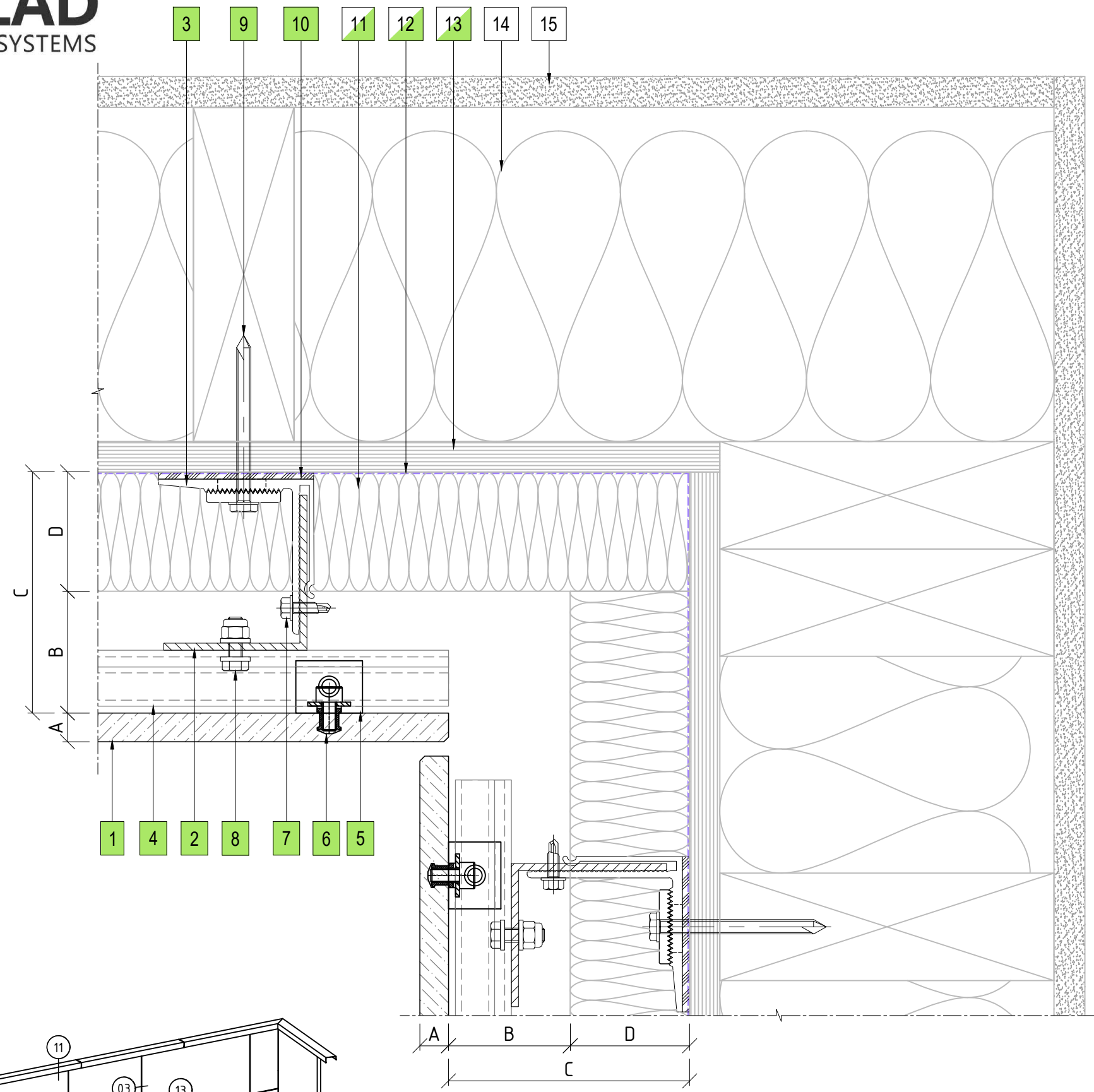
05 INTERNAL CORNER PANEL DETAIL ENCLAD™ PORCELAIN TILES
