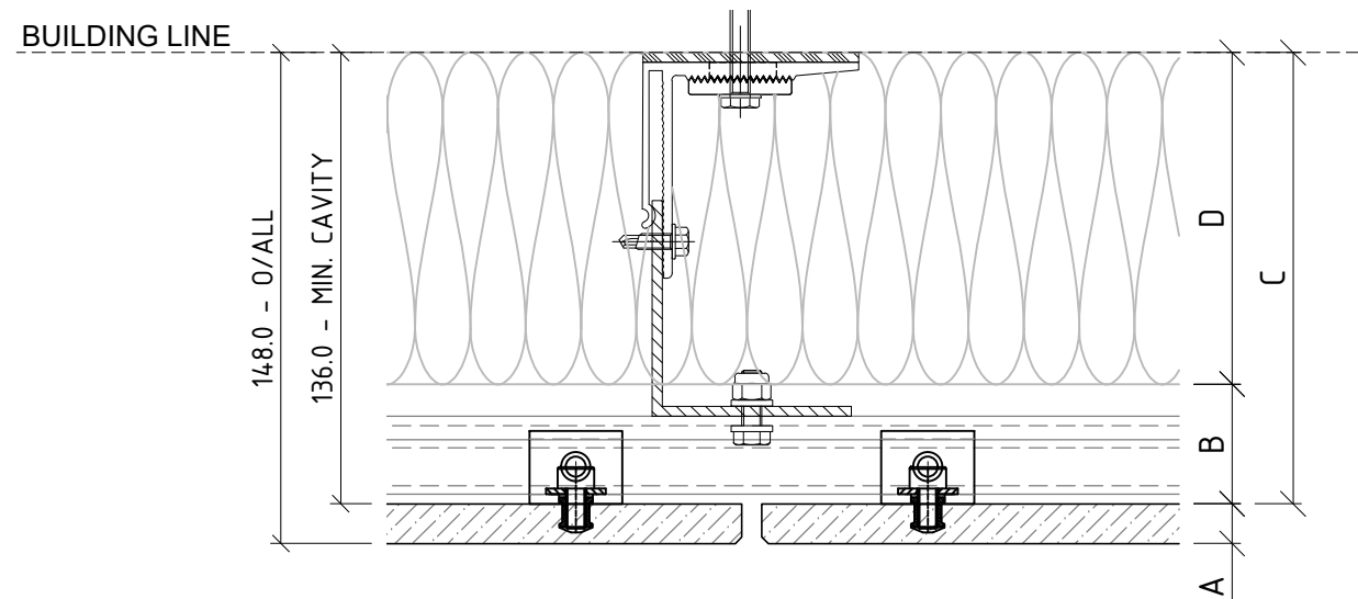
01 CAVITY SET OUT ENCLAD™ PORCELAIN TILES
