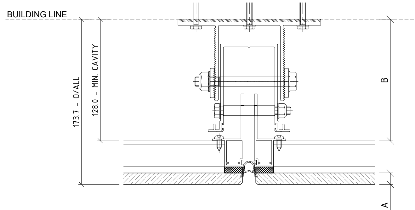
EN05 - FF MINIMUM SYSTEM CAVITY 128mm
