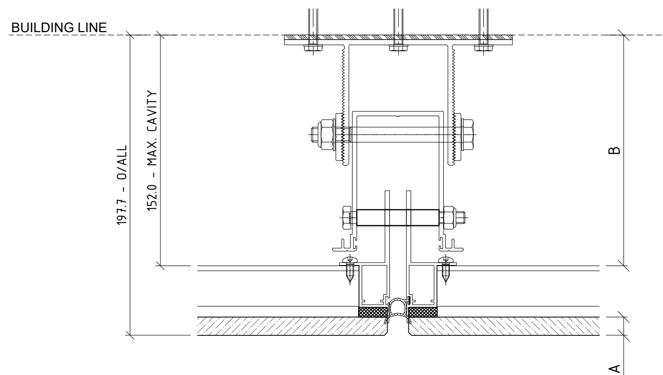
01 CAVITY SET OUT ENCLAD™ PORCELAIN TILES
