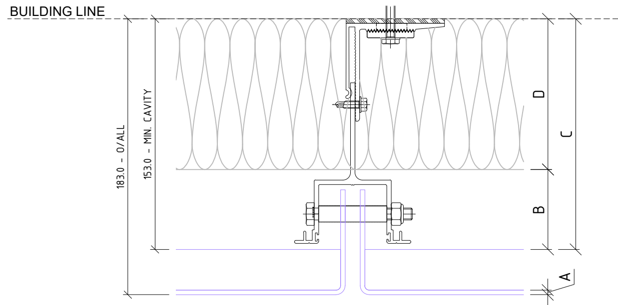
01 CAVITY SET OUT ENCLAD™ SOLID SHEET *
