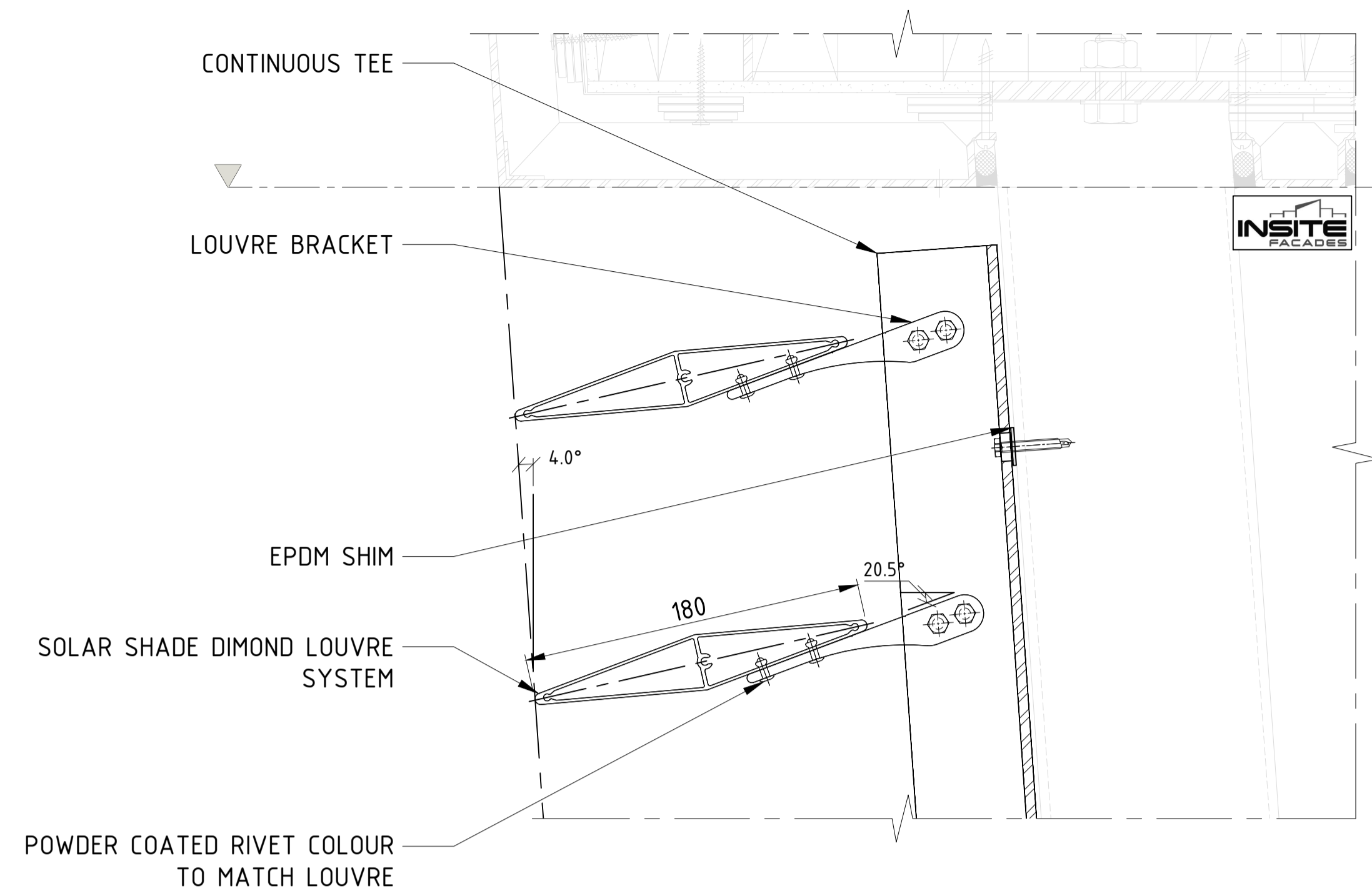
09 01 LOUVRE PARAPET DETAIL Scale 1 : 2.5
