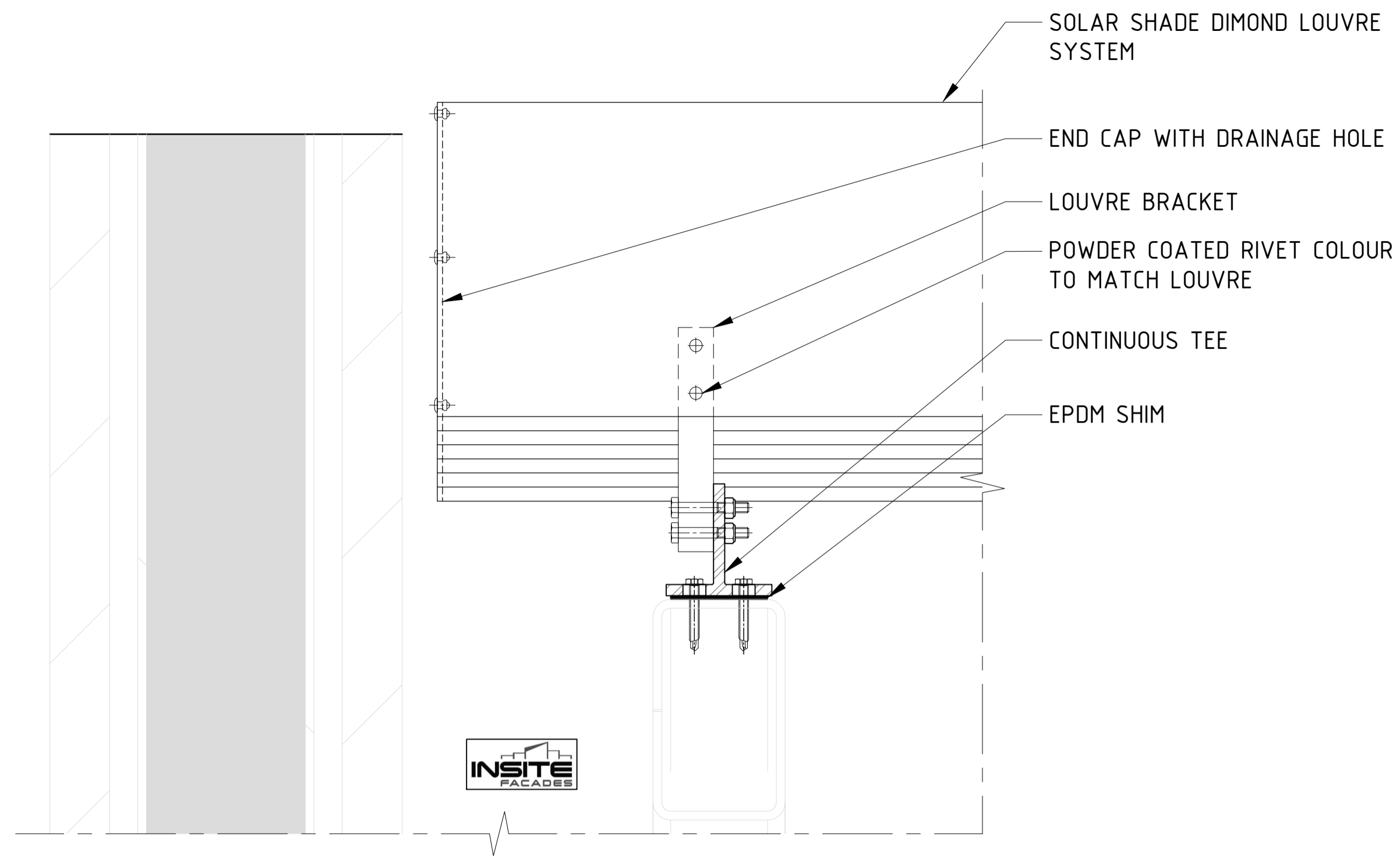
08 LOUVRE NORTH END DETAIL 01 Scale 1 : 2.5
