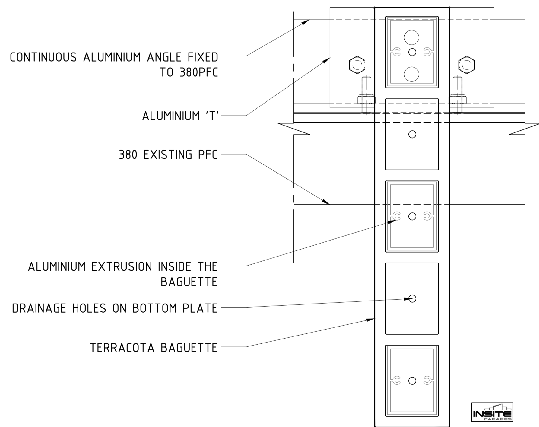
06 HORIZONTAL DETAIL Scale 1 : 2.5
