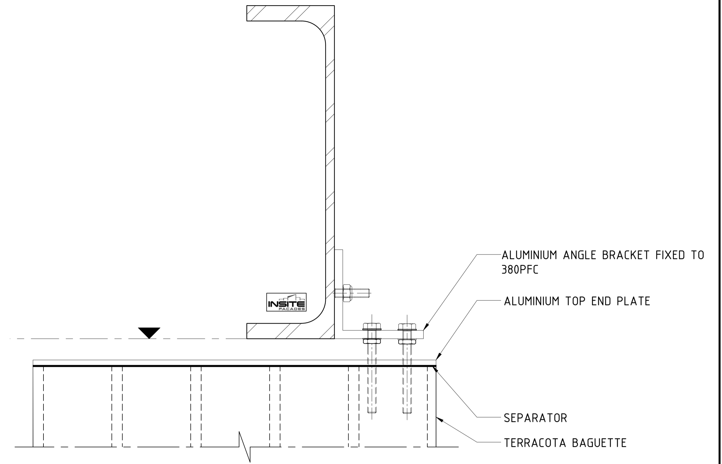
06 HEAD DETAIL Scale 1 : 2.5
