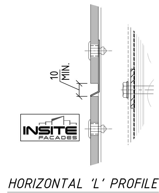
01 HORIZONTAL DETAIL Scale 1 : 2
